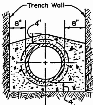
No. 1 CONCRETE ENCASEMENT
