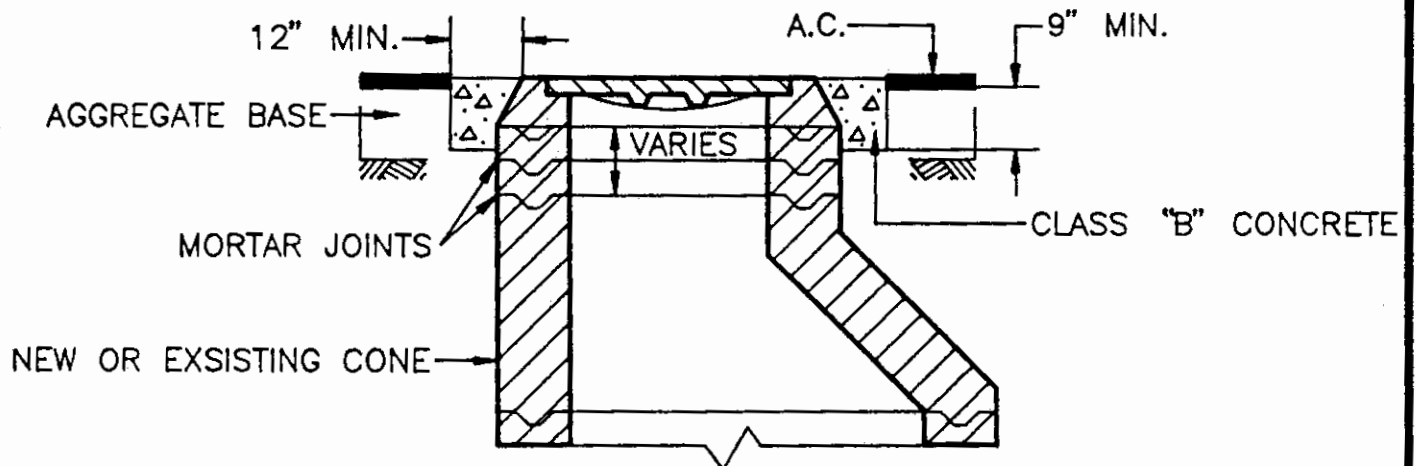
CROSS-SECTION
