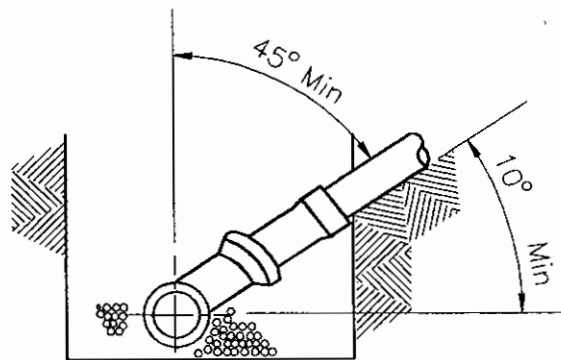
PROFILE DETAIL
