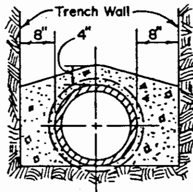
No. 2 CONCRETE ENCASEMENT
