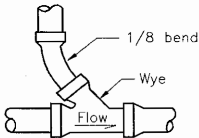
WYE DETAIL
