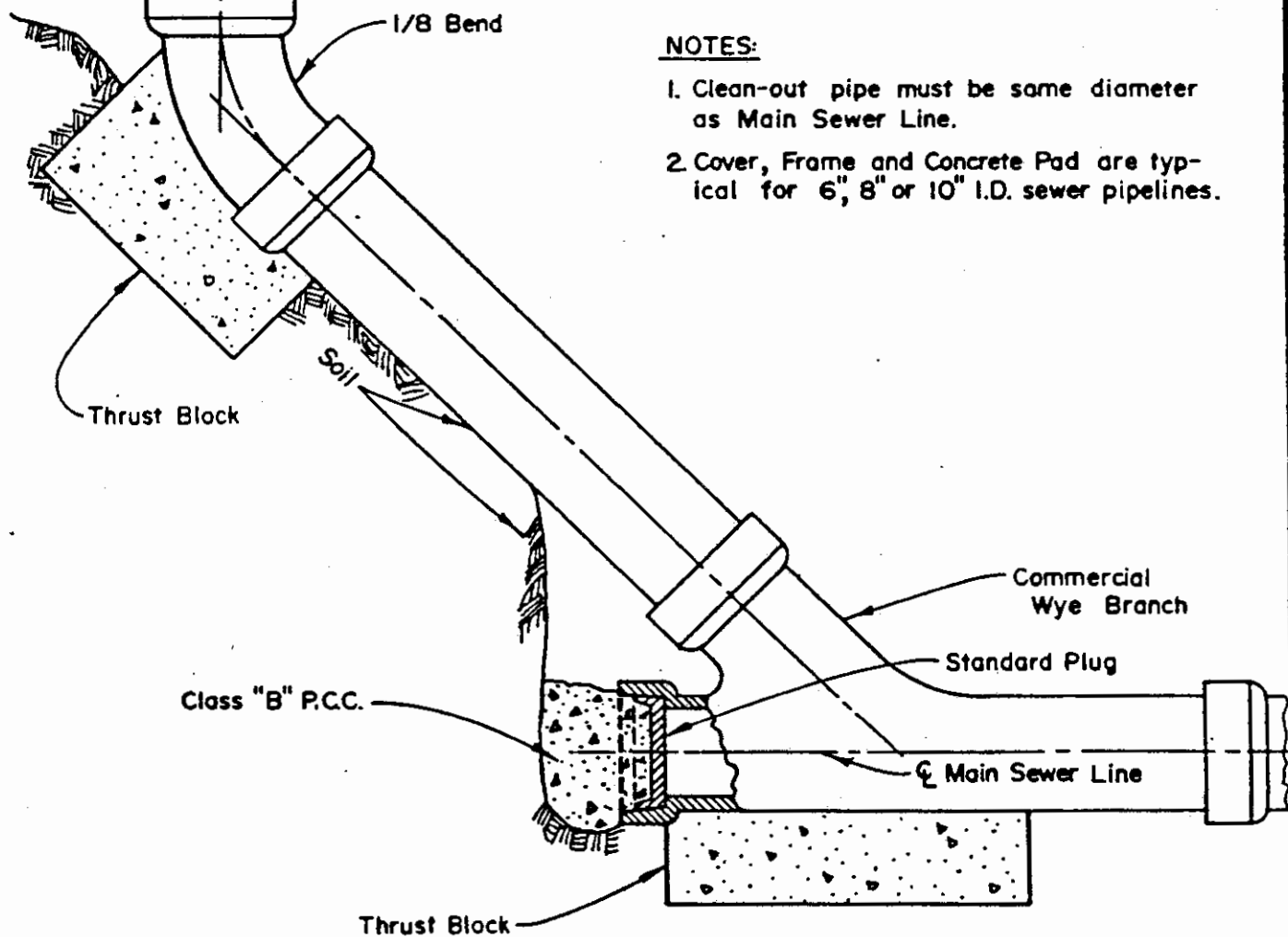
STANDARD CLEAN-OUT
