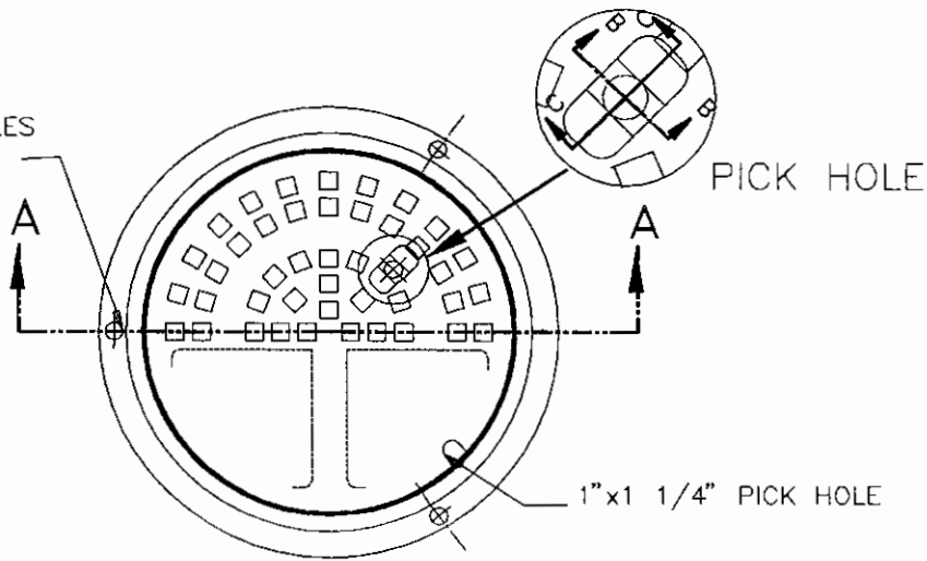
PLAN VIEW
