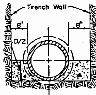
CONCRETE CRADLE
