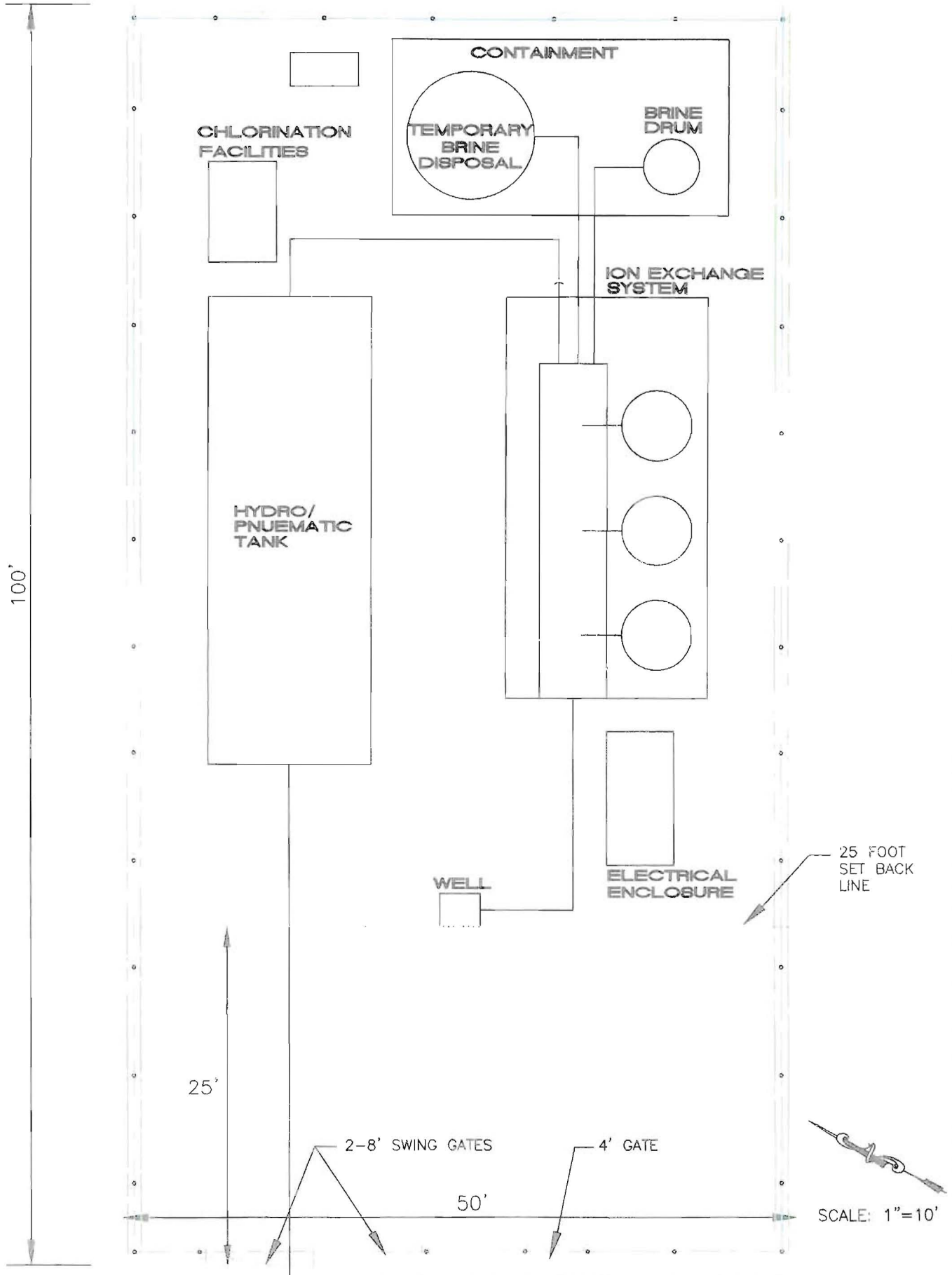
TYPICAL ION EXCHANGE PROCESS LAYOUT - WELL SITE WATER SUPPLY STUDY CUTLER-OROSI AREA
