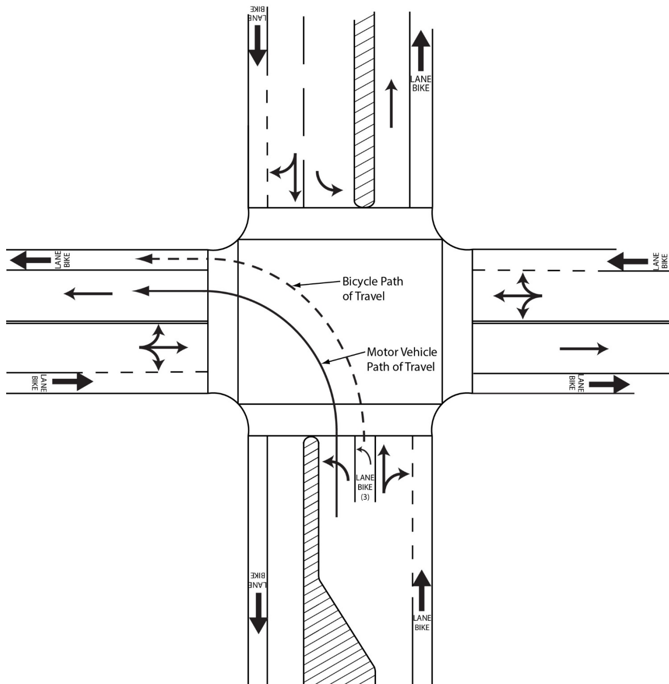
Figure 403.6B Bicycle Left-Turn-Only Lane
