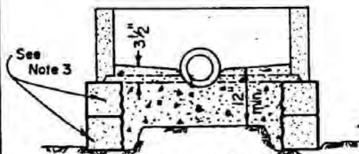
SECTION \frac{C}{5}
