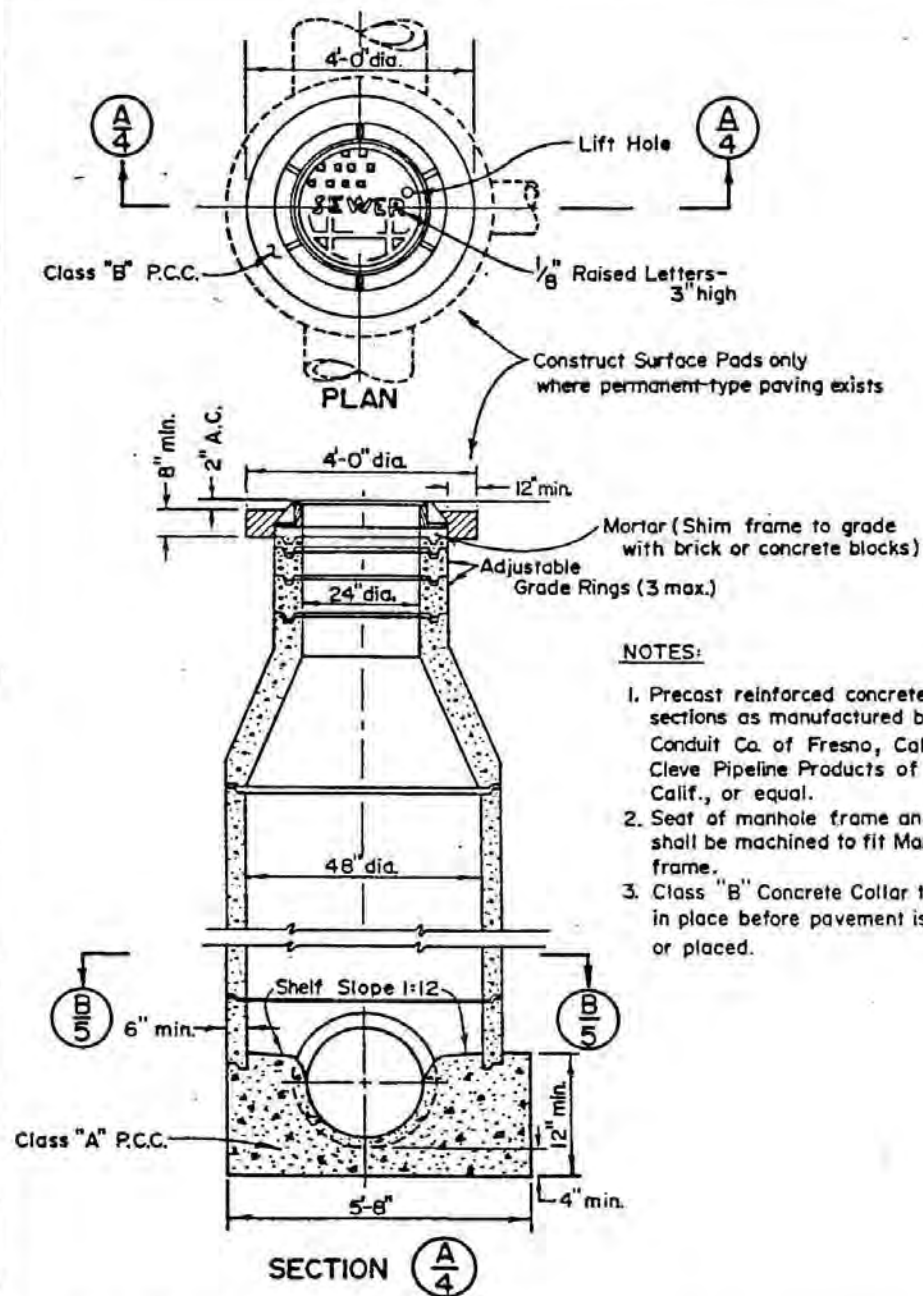
SANITARY SEWER MANHOLE DETAIL SHEET NO. 1
